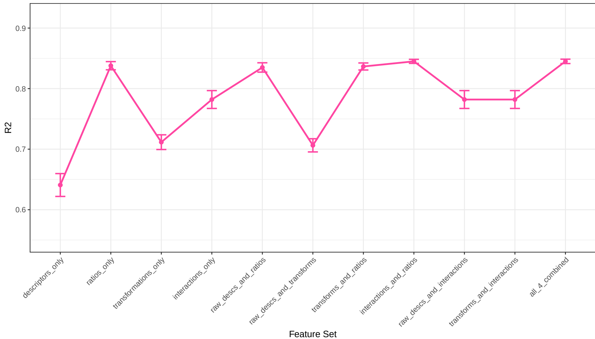
Ridge Regression R2 Across Feature Sets
