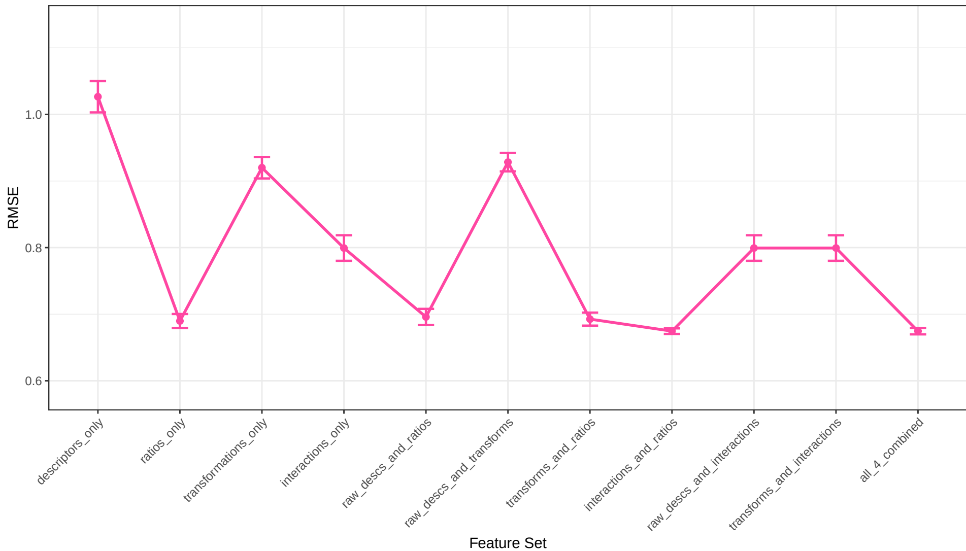
Ridge Regression RMSE Across Feature Sets
