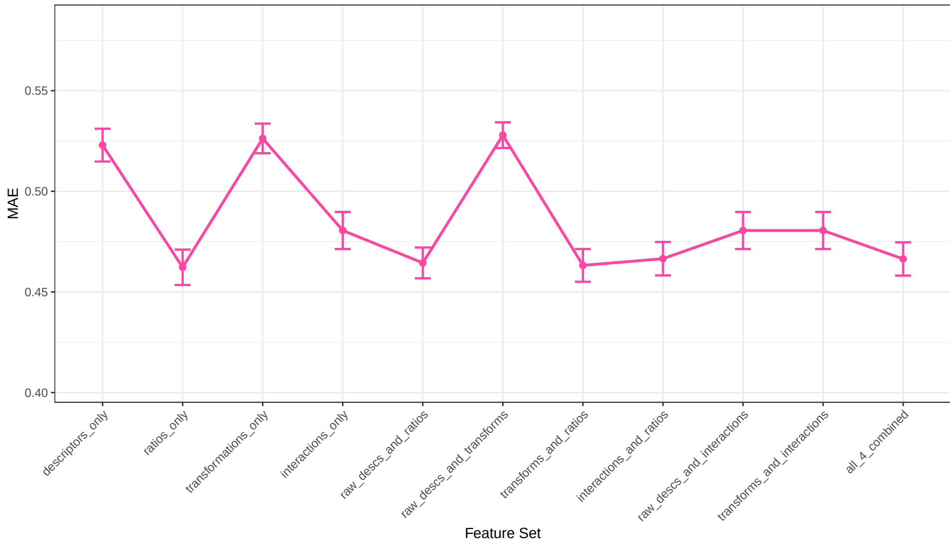
Stacking Regression MAE Across Feature Sets
