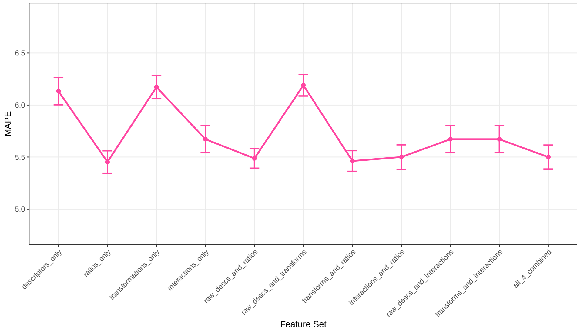
Stacking Regression MAPE Across Feature Sets
