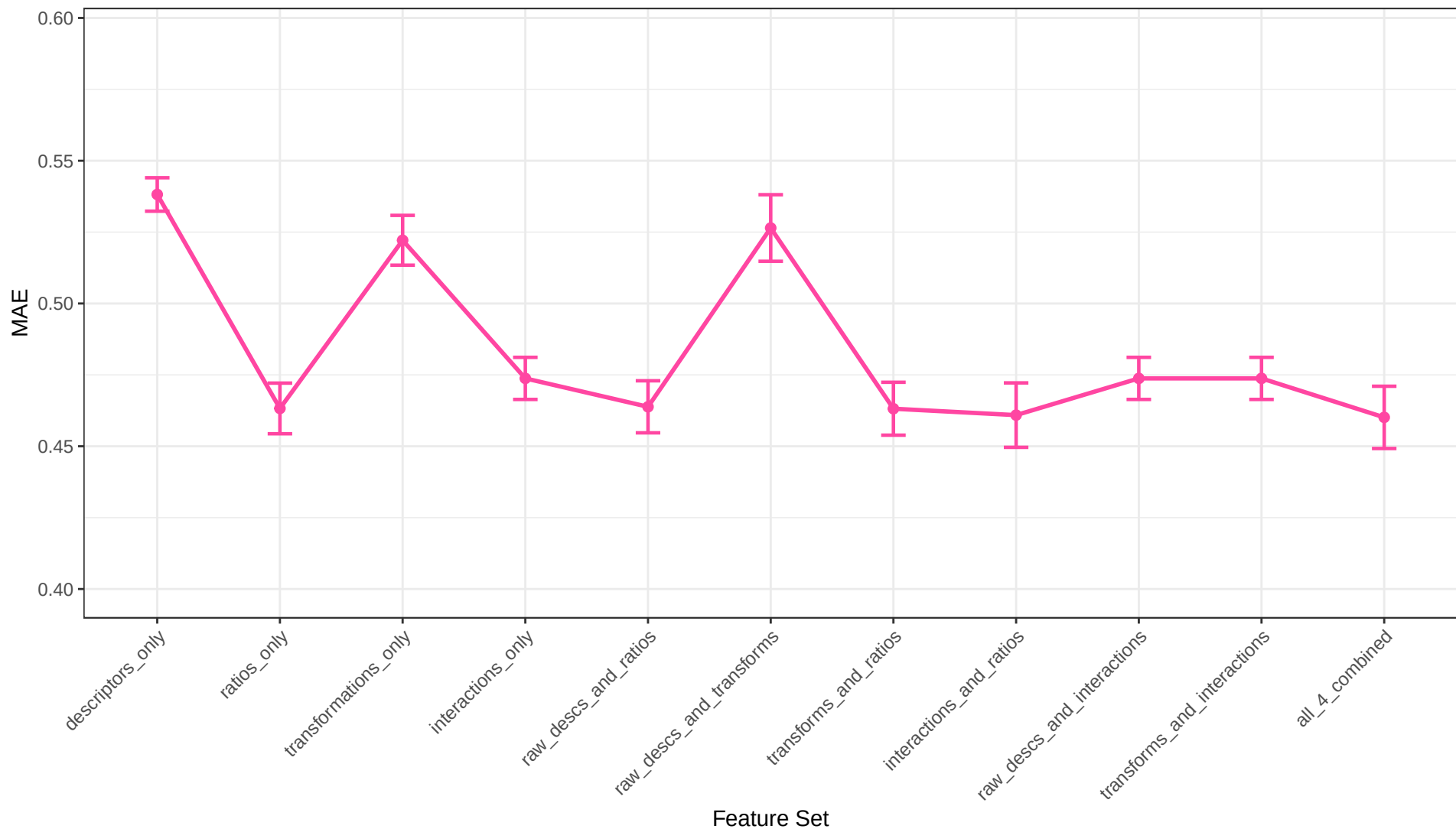
Support Vector Regression MAE Across Feature Sets
