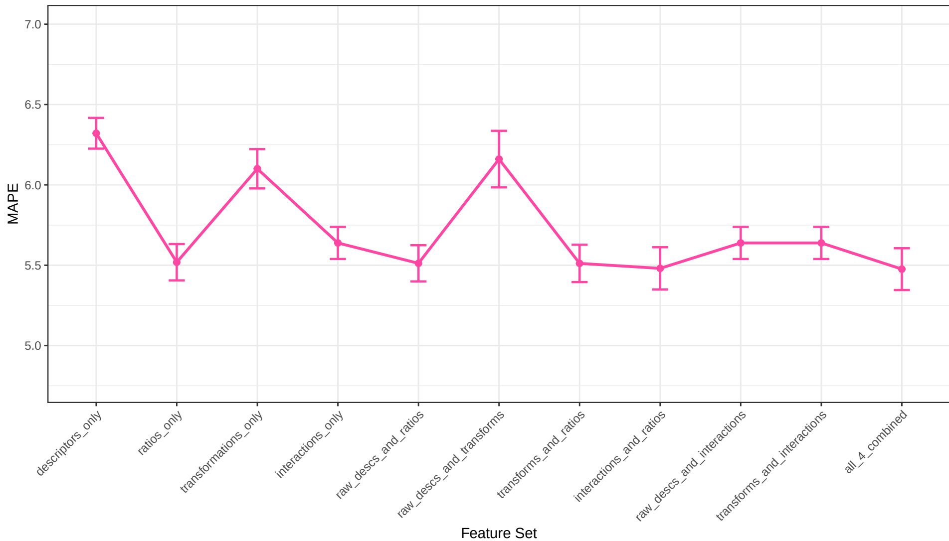
Support Vector Regression MAPE Across Feature Sets
