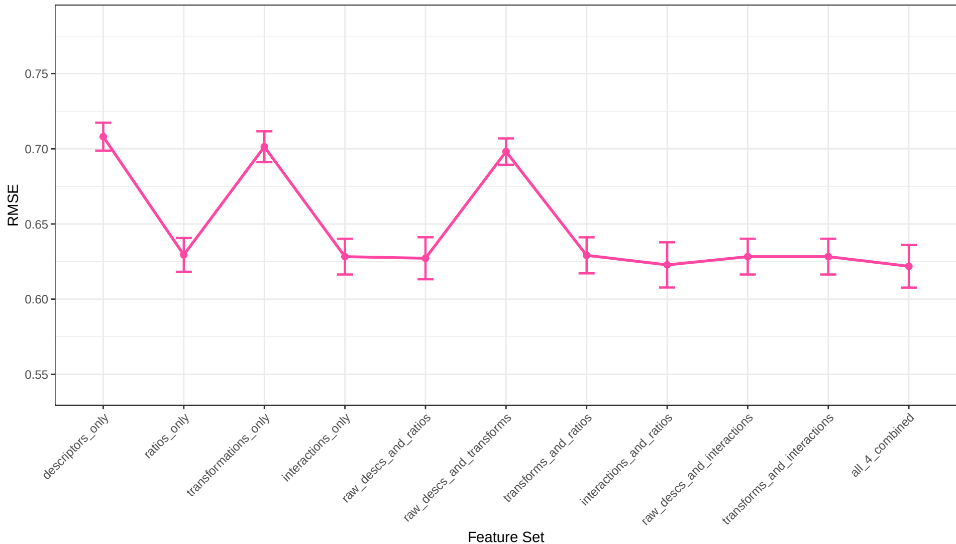
Support Vector Regression RMSE Across Feature Sets
