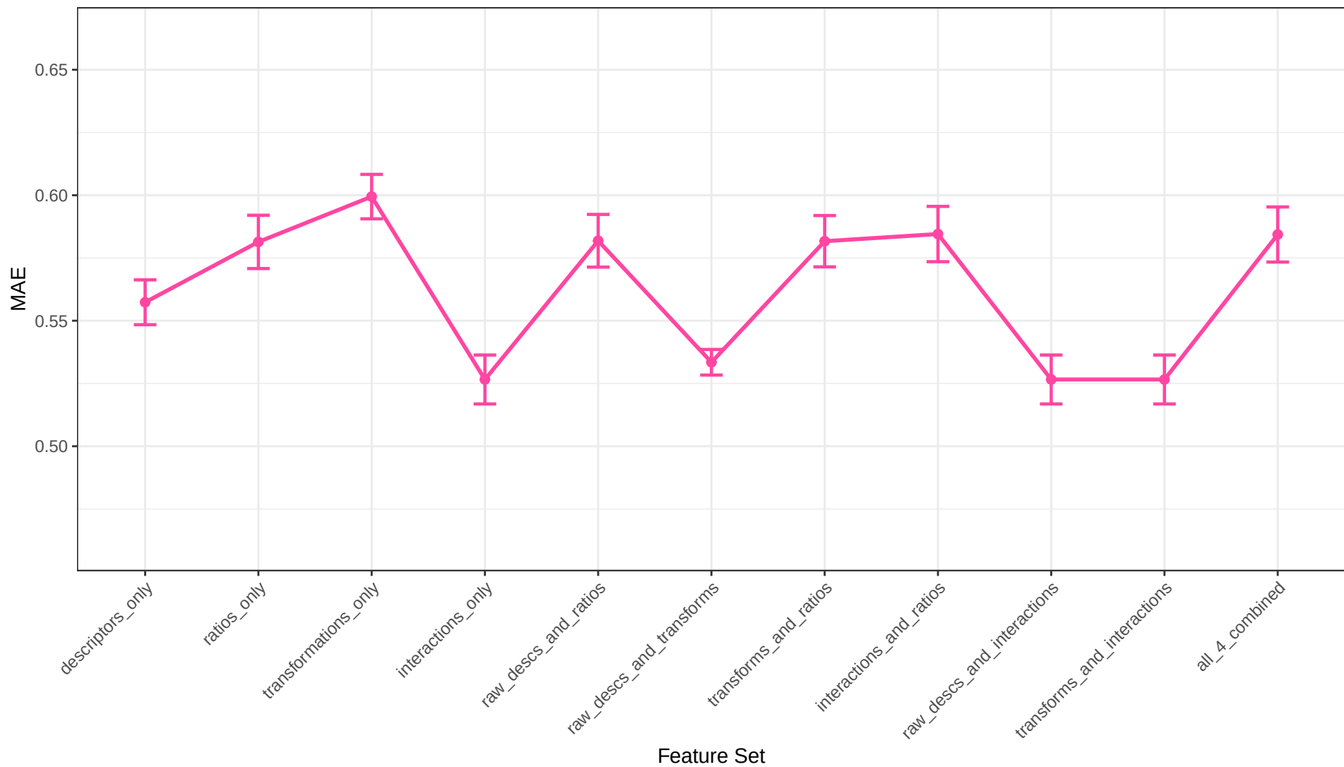
Voting Regression MAE Across Feature Sets
