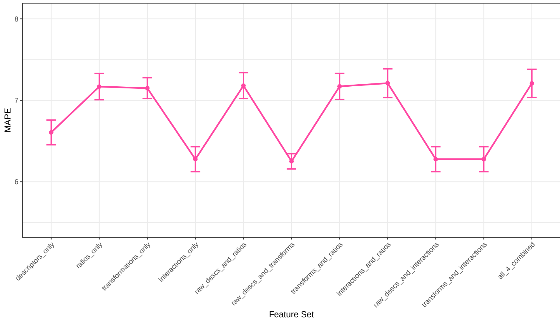
Voting Regression MAPE Across Feature Sets
