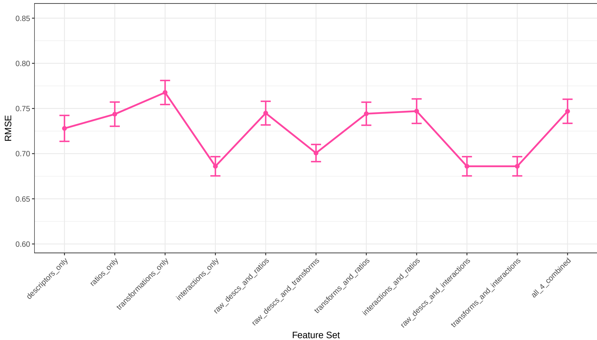
Voting Regression RMSE Across Feature Sets
