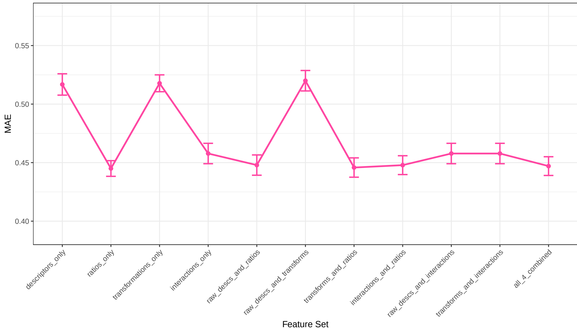
XGBoost Regression MAE Across Feature Sets
