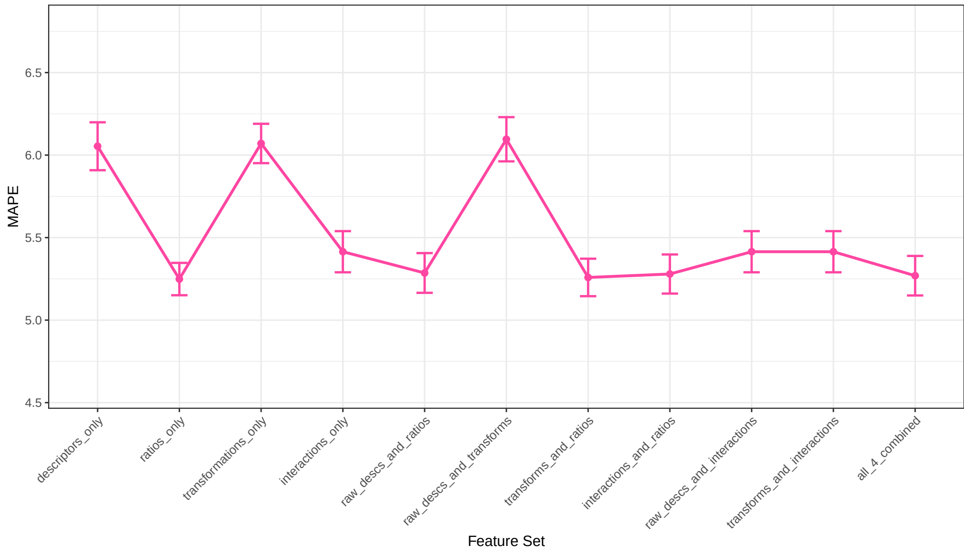
XGBoost Regression MAPE Across Feature Sets
