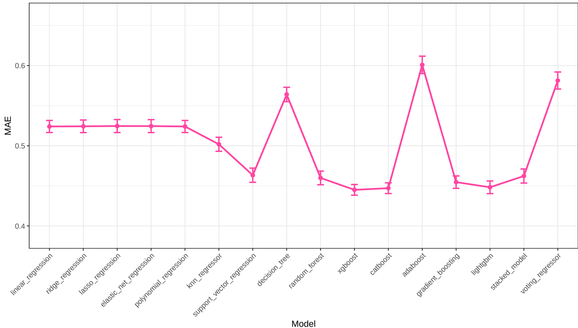
Ratios Only MAE Across Models
