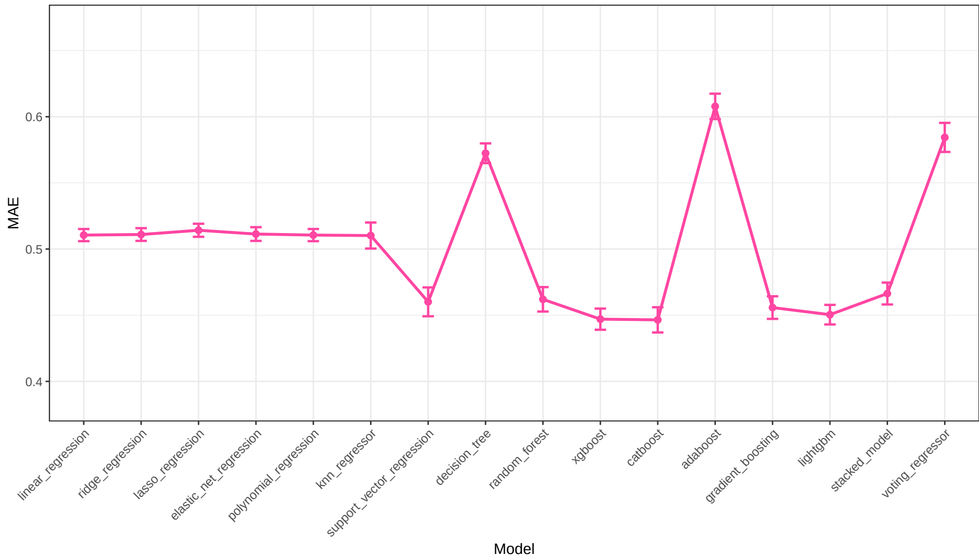
Combined MAE Across Models
