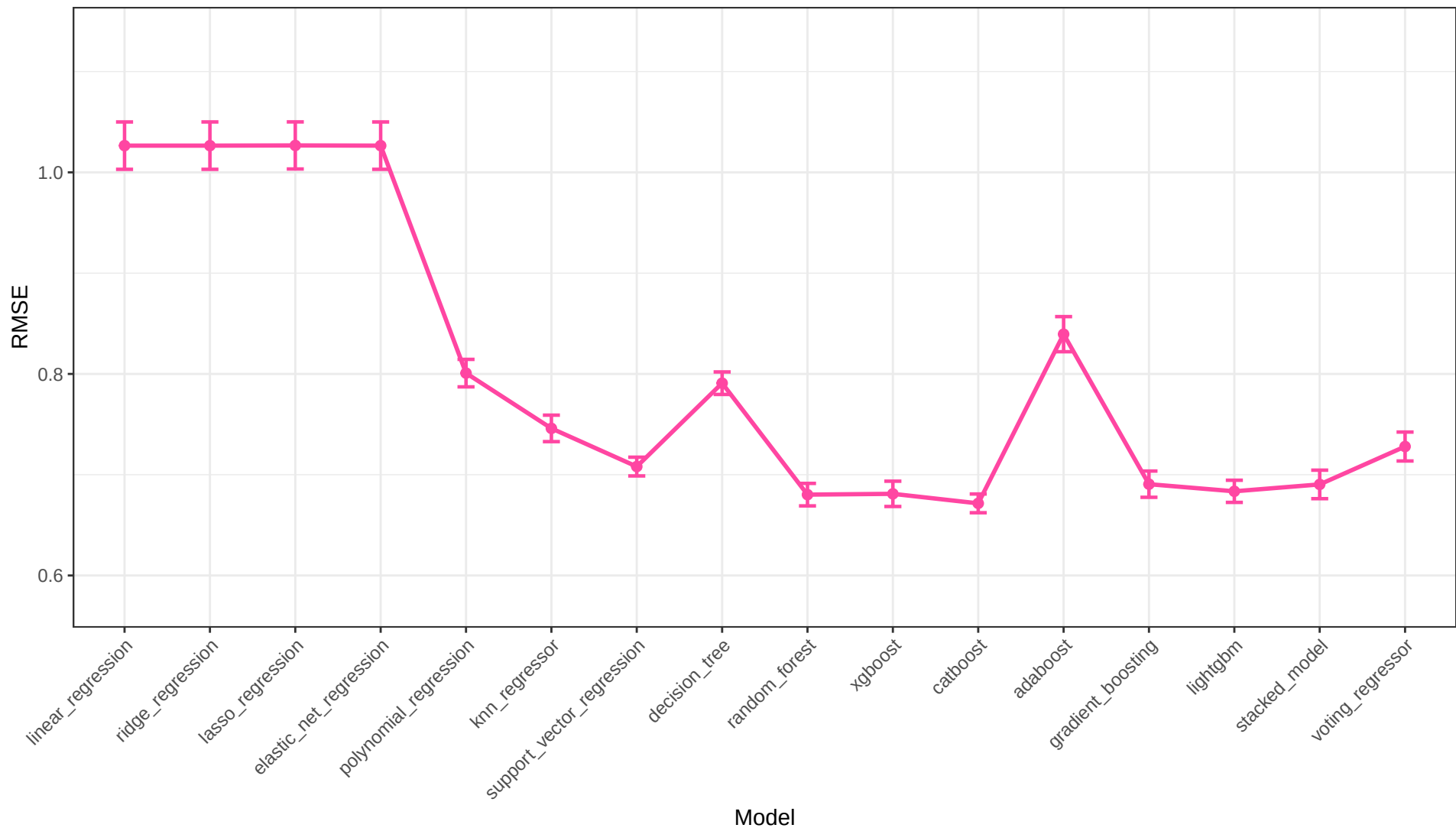
Descriptors Only RMSE Across Models
