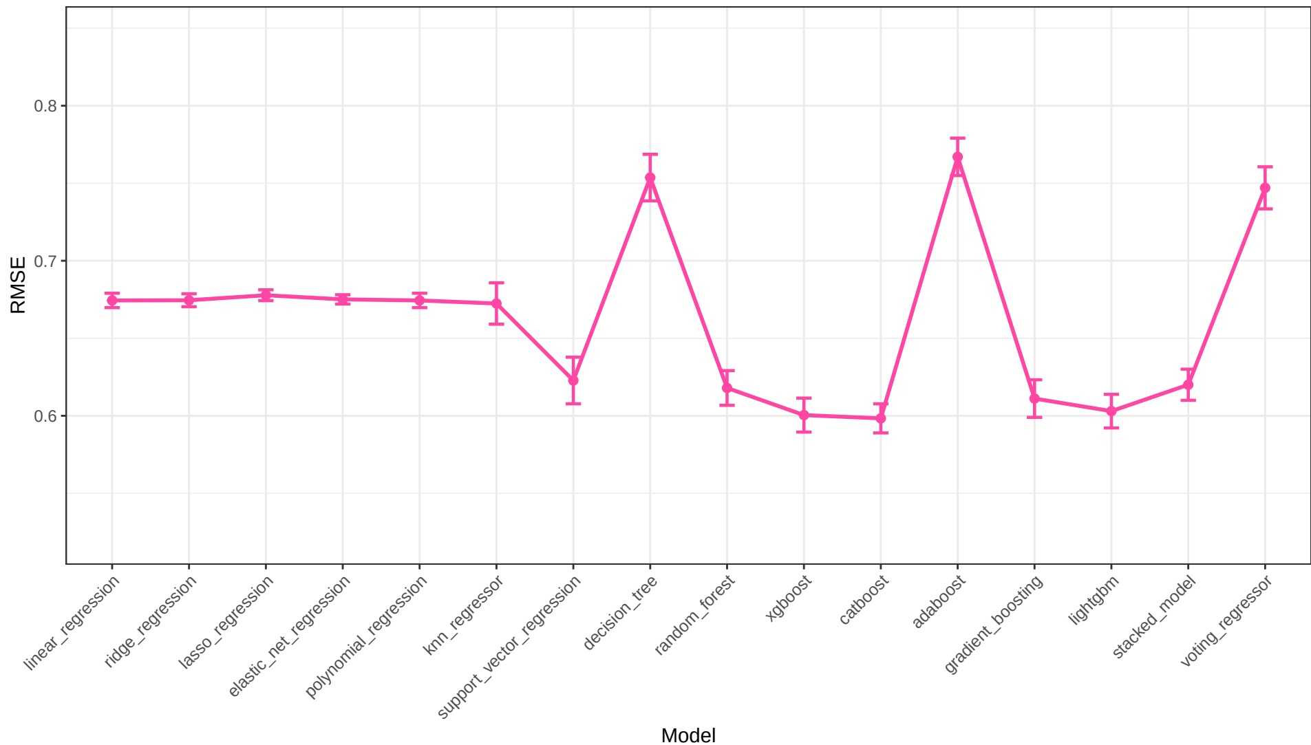
Ratios and Interactions RMSE Across Models
