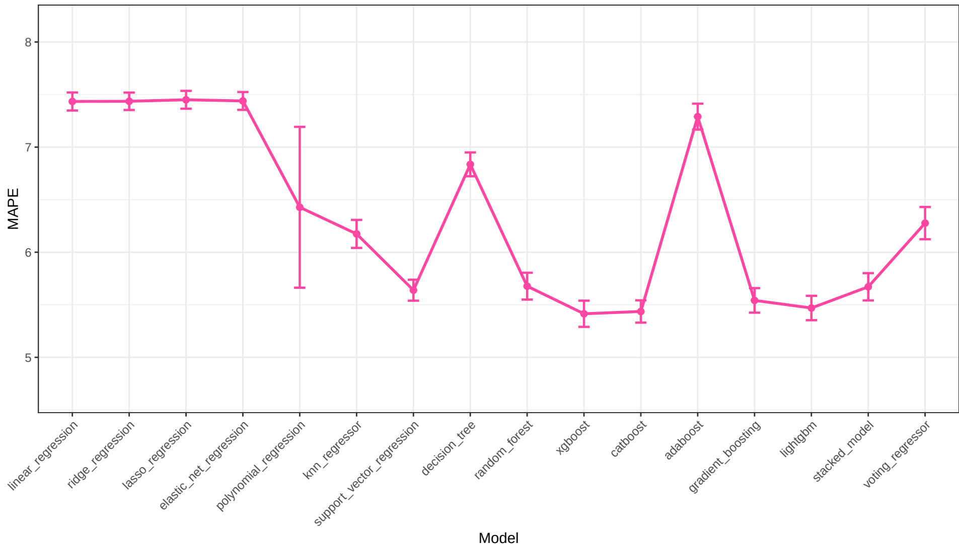
Interactions Only MAPE Across Models
