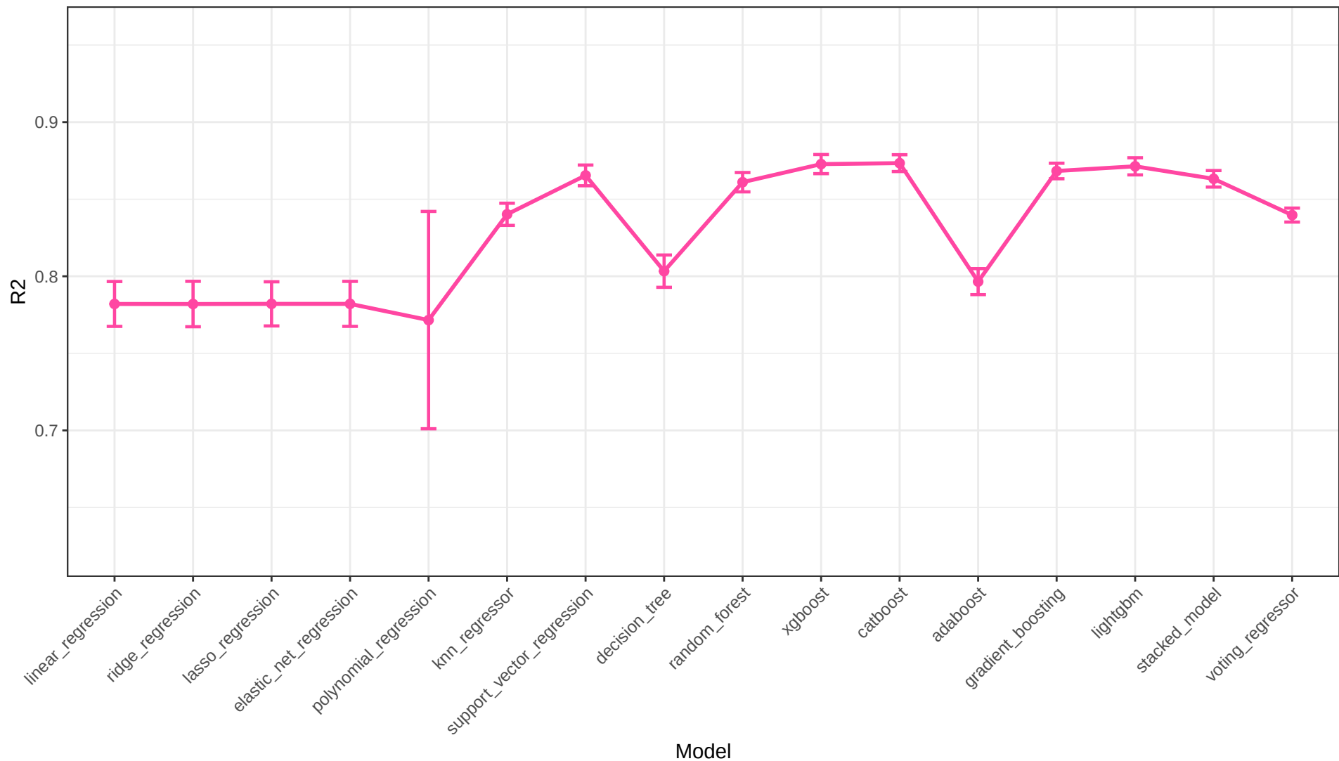
Interactions Only R2 Across Models
