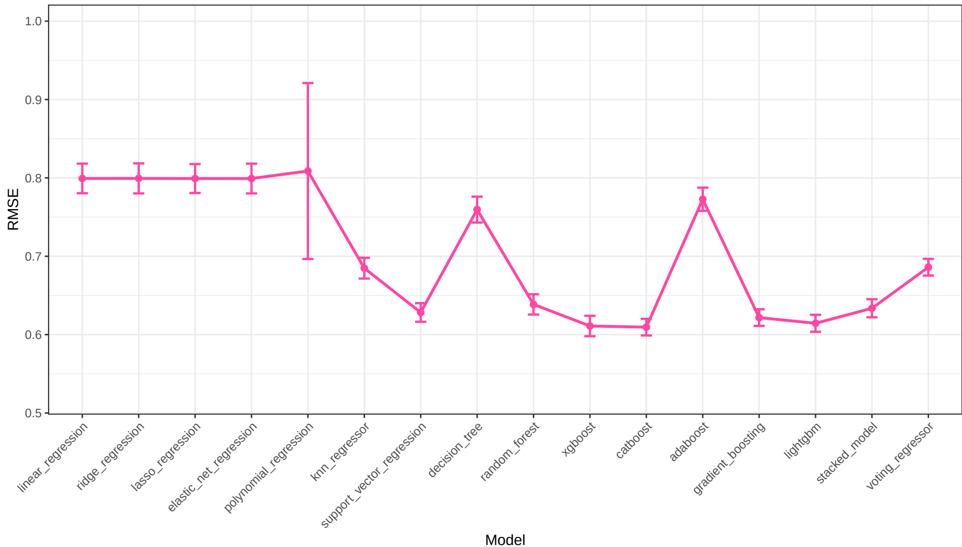
Interactions Only RMSE Across Models
