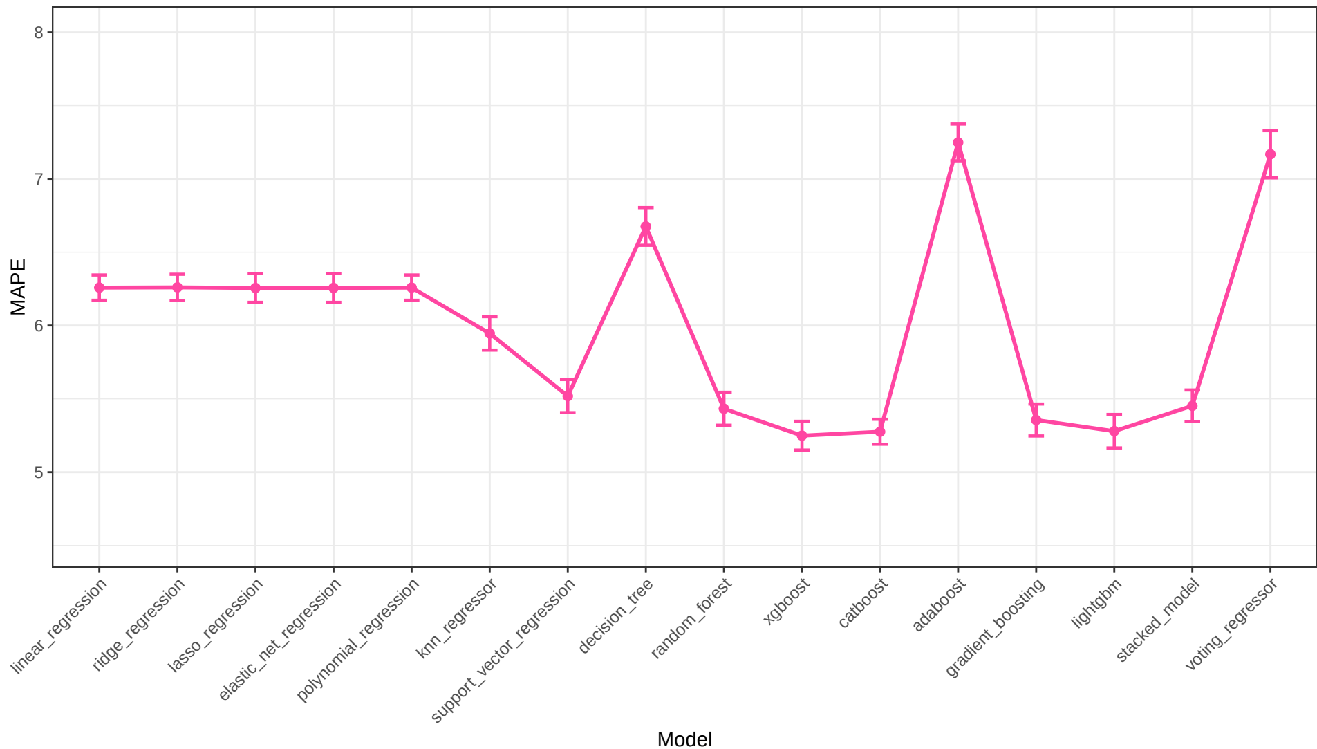
Ratios Only MAPE Across Models
