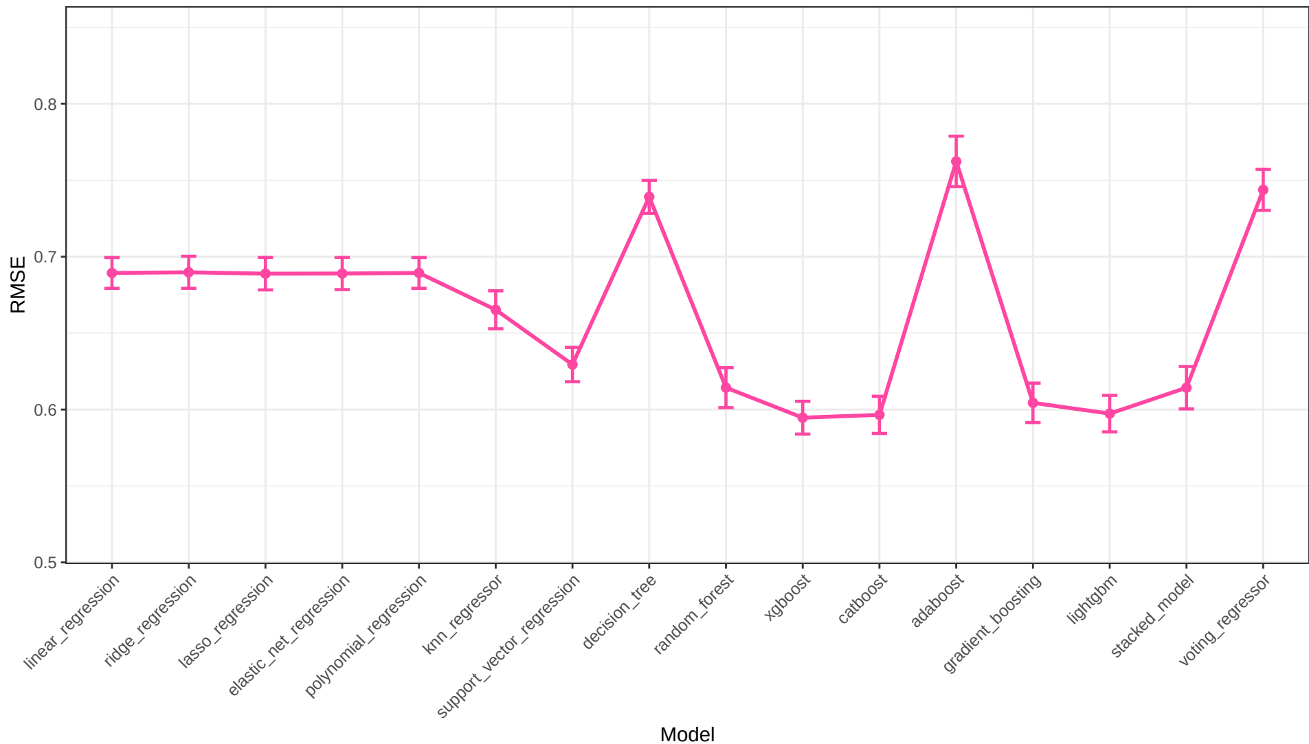
Ratios Only RMSE Across Models
