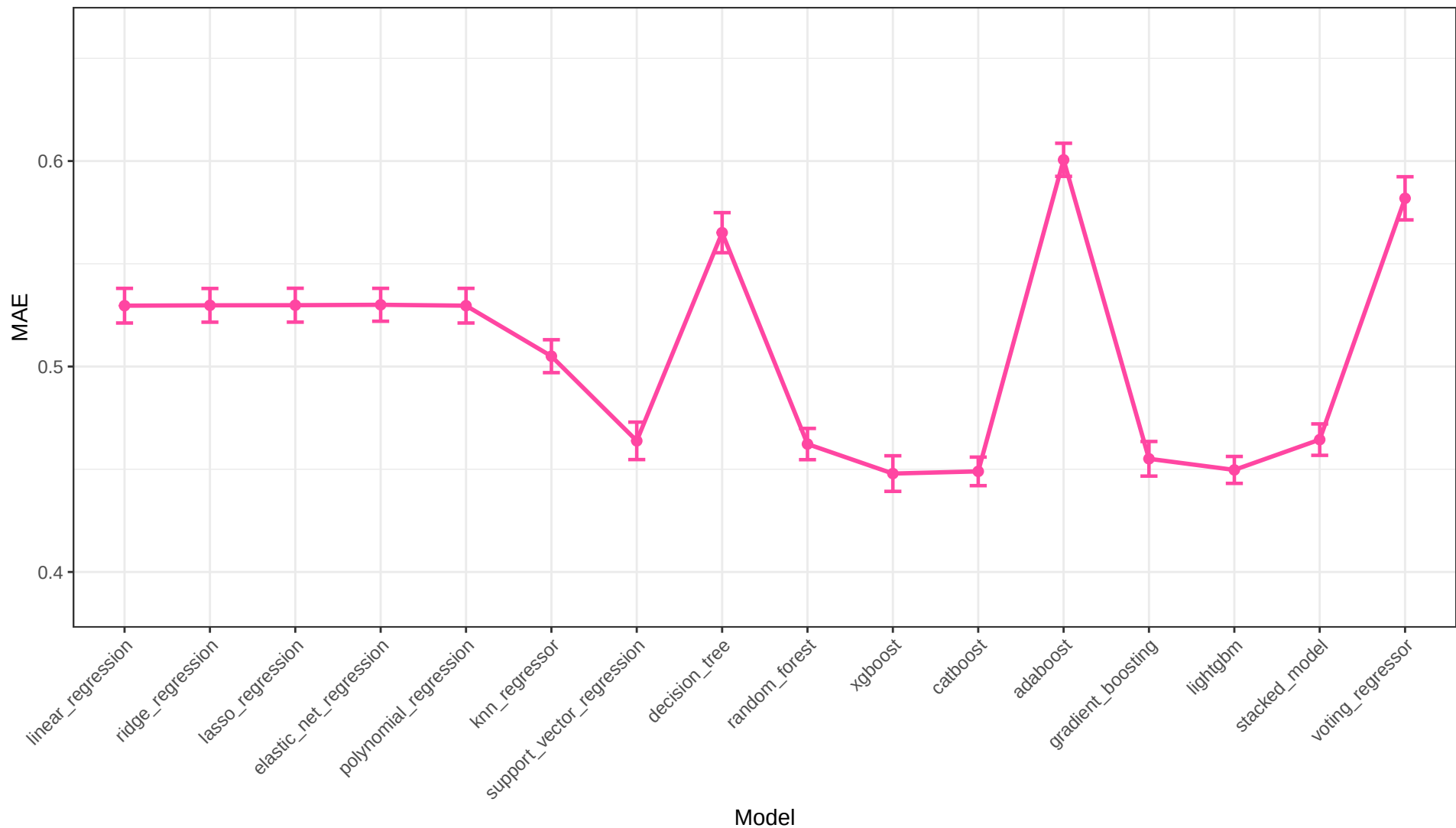
Raw Descriptors and Ratios MAE Across Models
