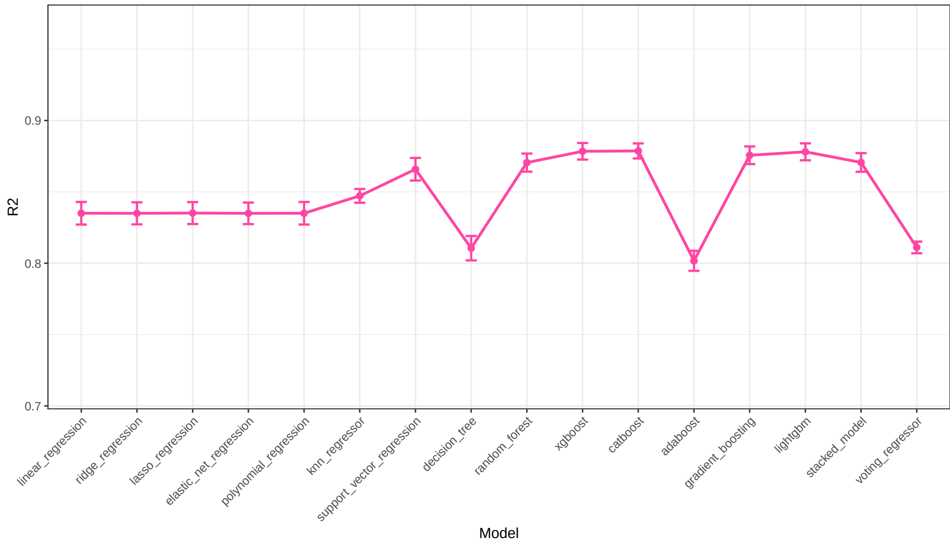
Raw Descriptors and Ratios R2 Across Models
