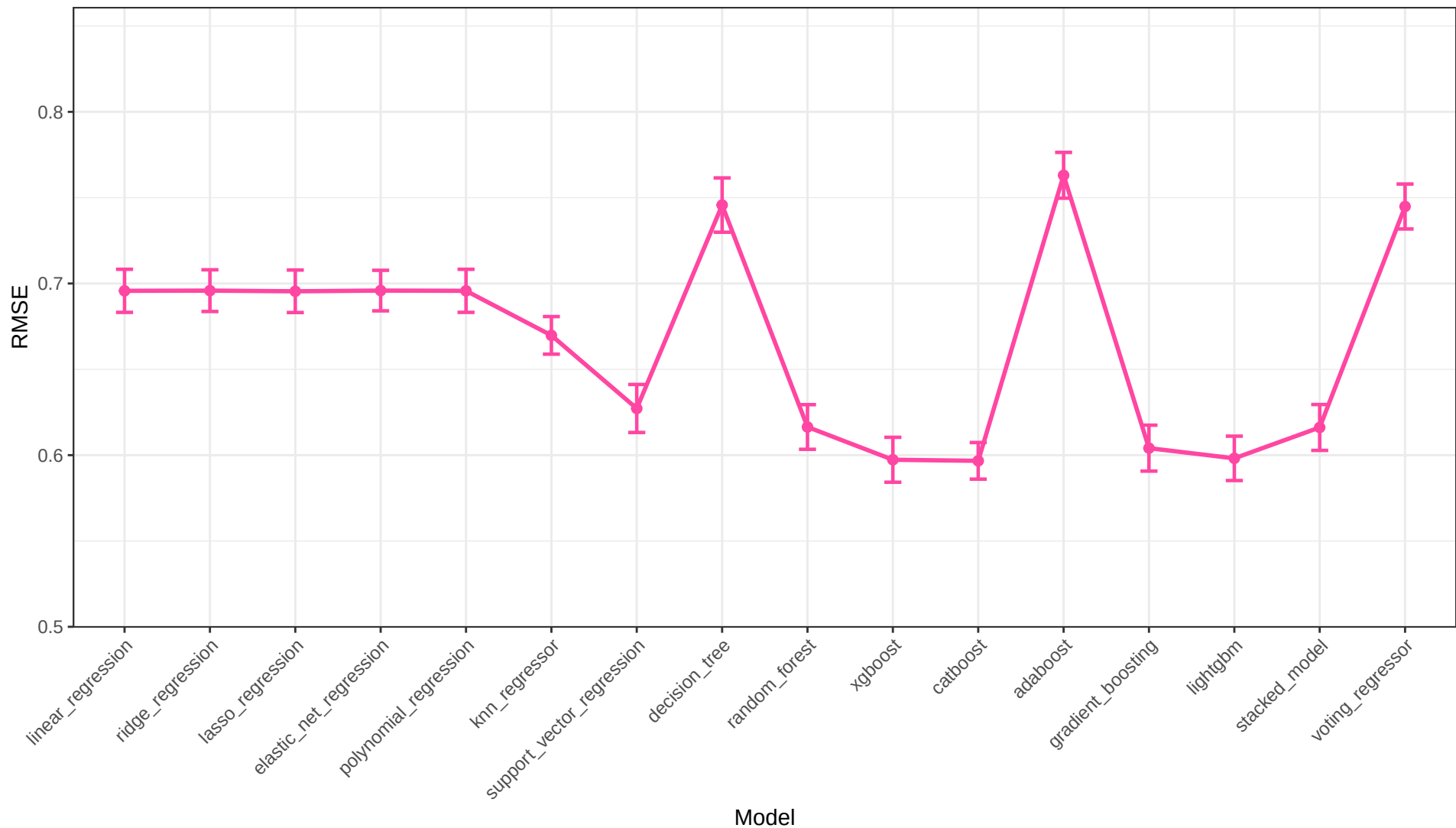
Raw Descriptors and Ratios RMSE Across Models
