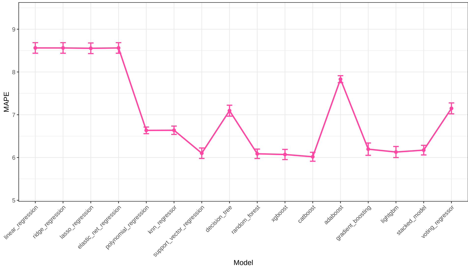
Transformations Only MAPE Across Models
