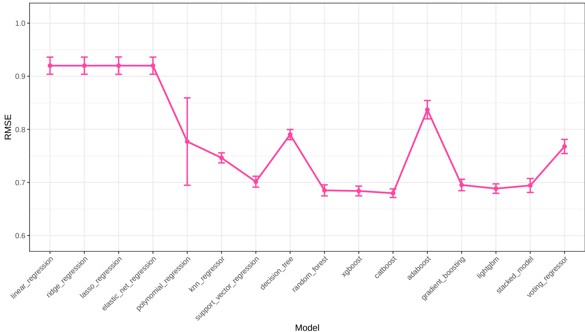
Transformations Only RMSE Across Models
