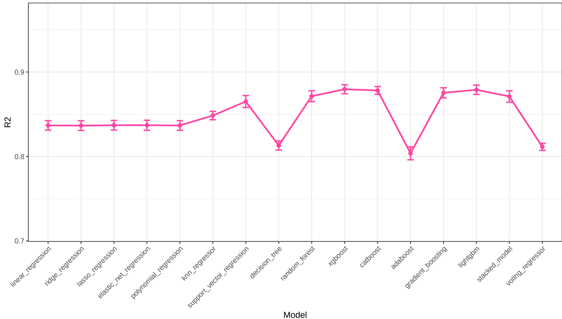
Ratios and Transformations R2 Across Models
