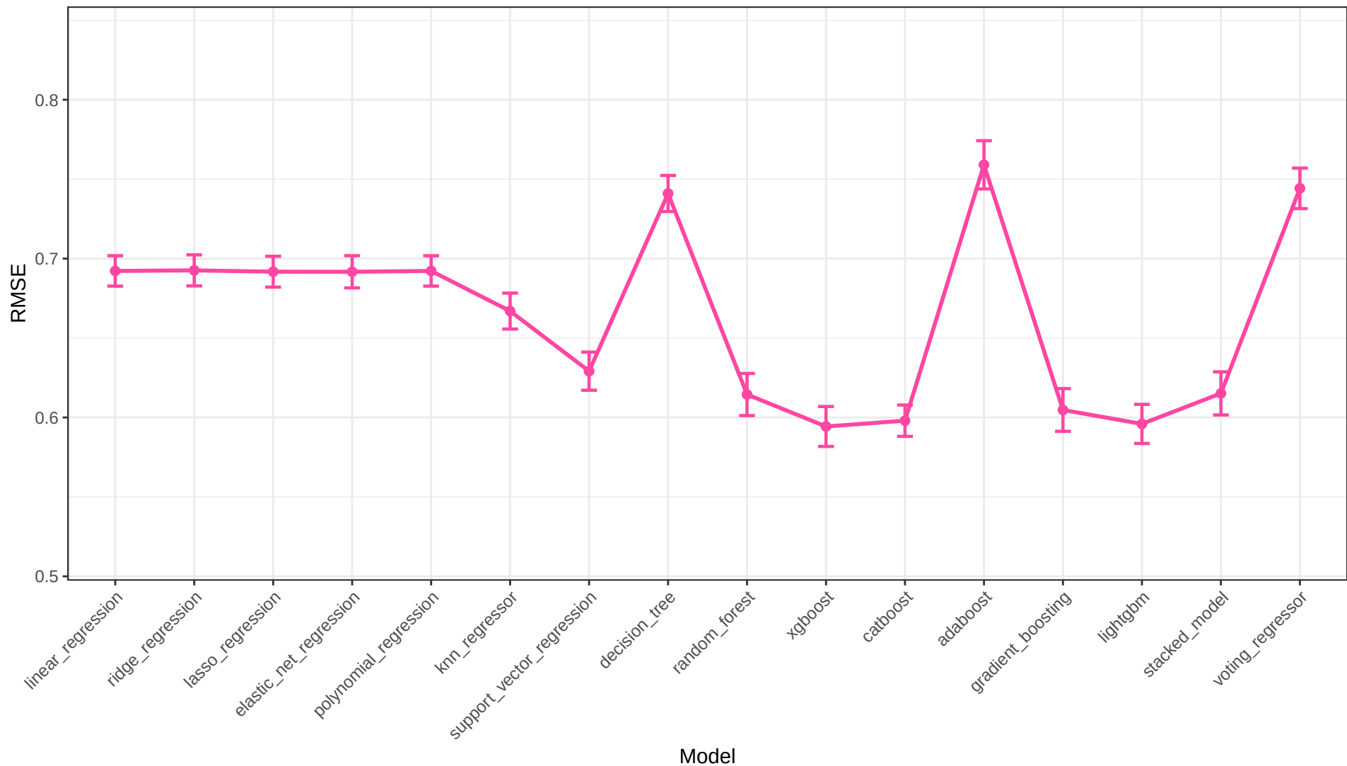
Ratios and Transformations RMSE Across Models
