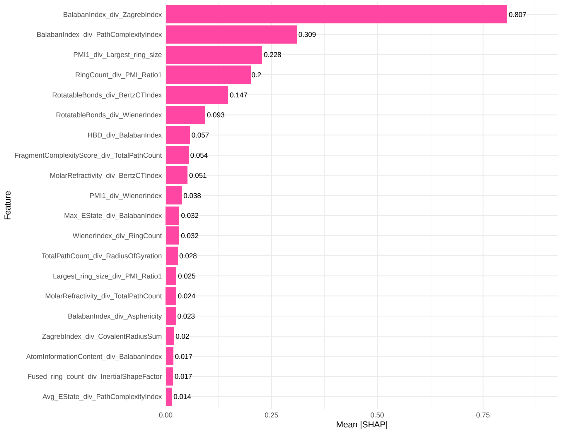
SHAP Feature Importances: Decision Tree Regression
