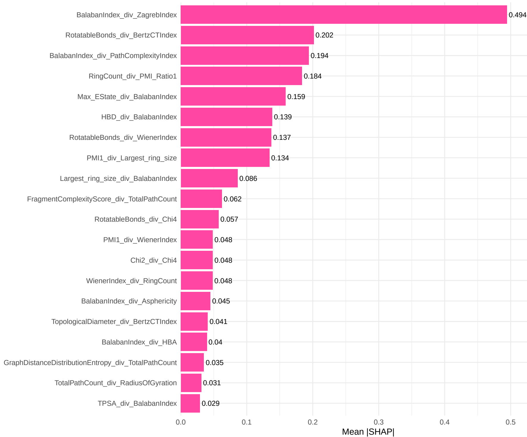
SHAP Feature Importances: Gradient Boosting Regression
