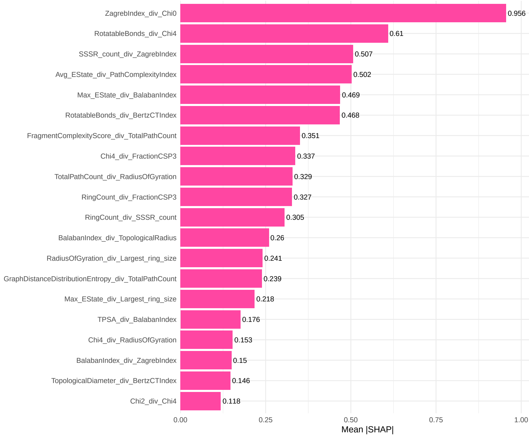
SHAP Feature Importances: Lasso Regression
