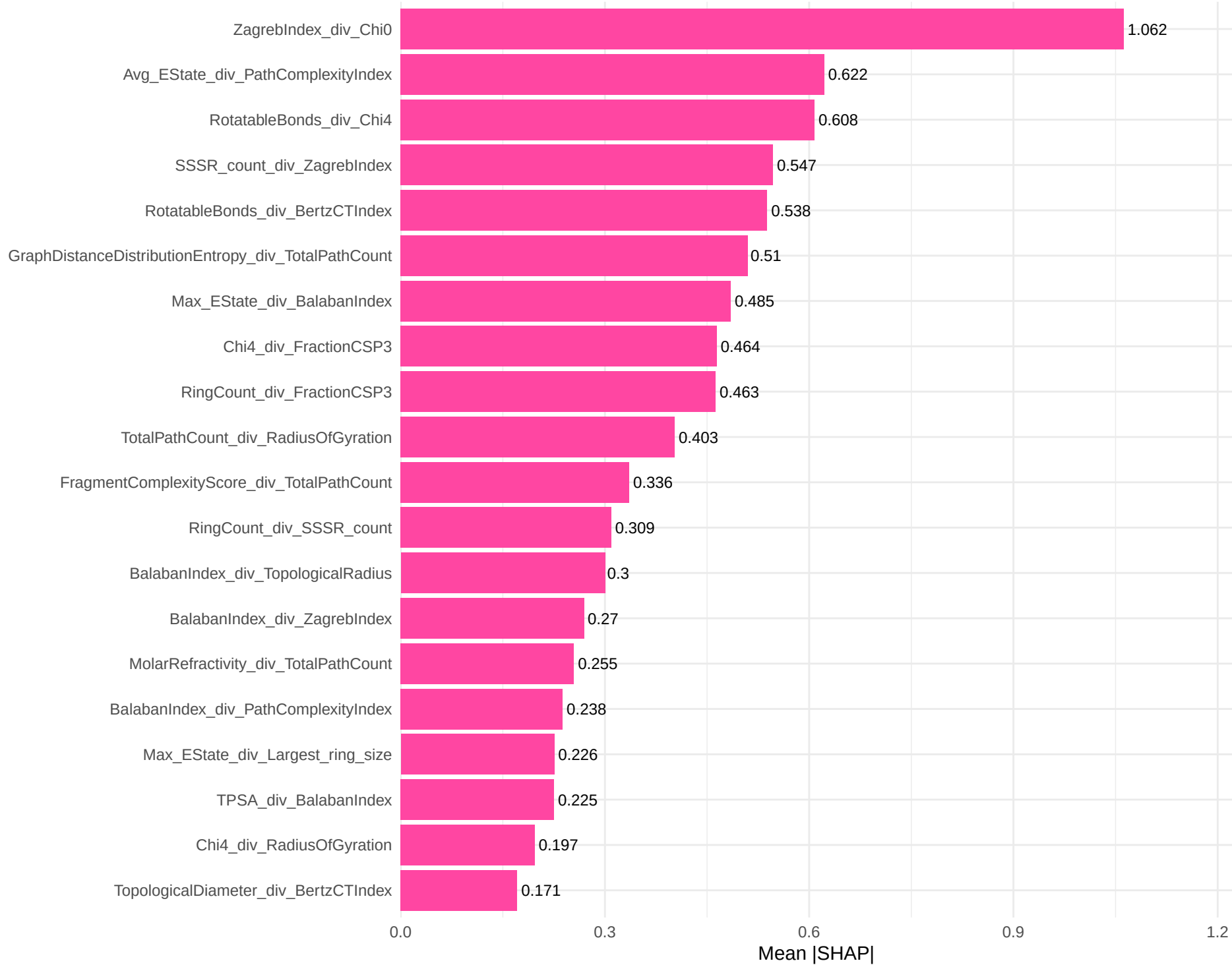
SHAP Feature Importances: Linear Regression
