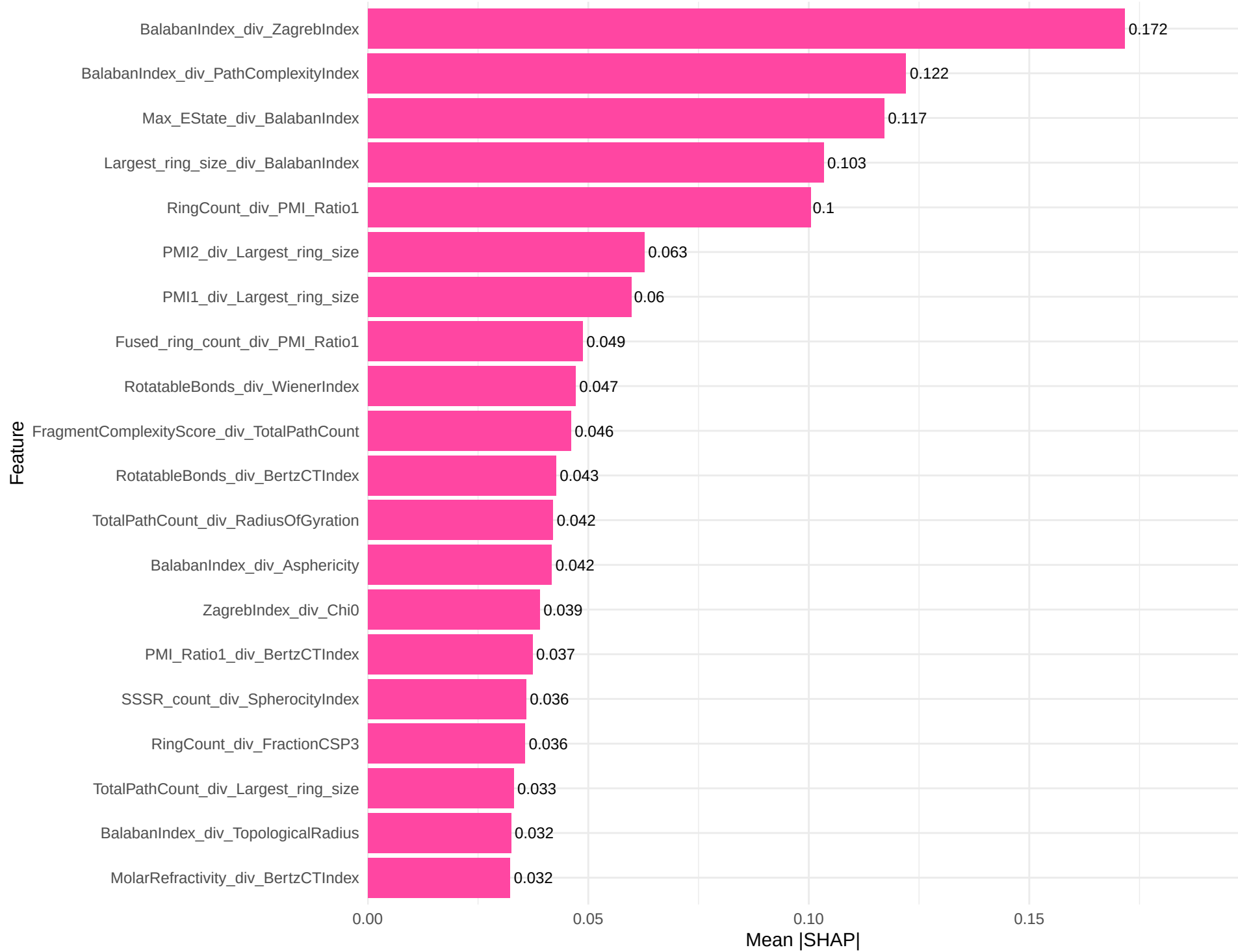
SHAP Feature Importances: Random Forest Regression
