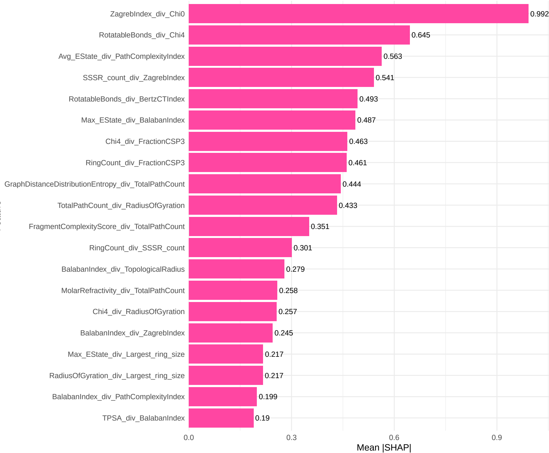
SHAP Feature Importances: Ridge Regression
