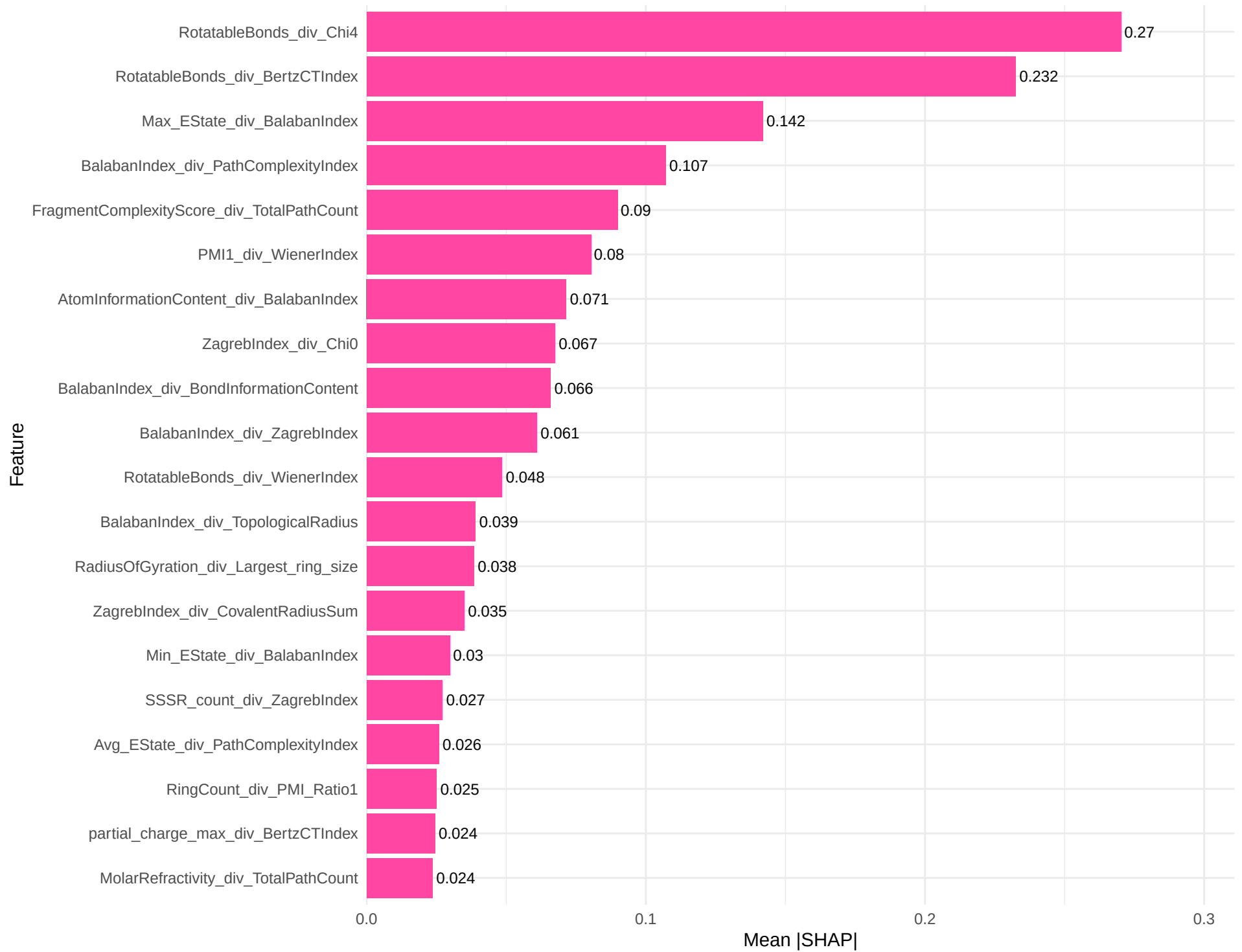
SHAP Feature Importances: Support Vector Regression
