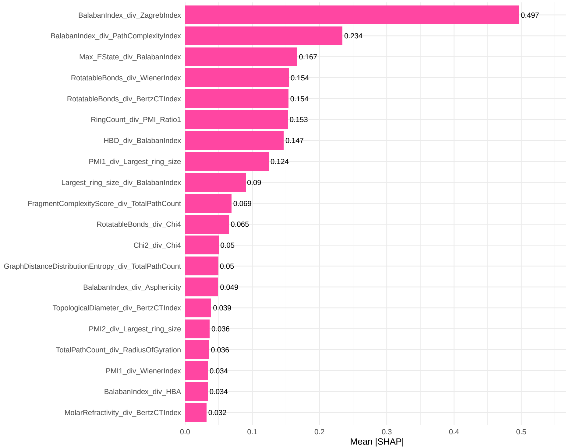
SHAP Feature Importances: XGBoost Regression
