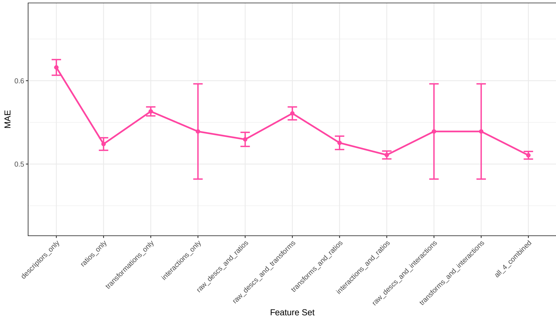
Polynomial Regression MAE Across Feature Sets
