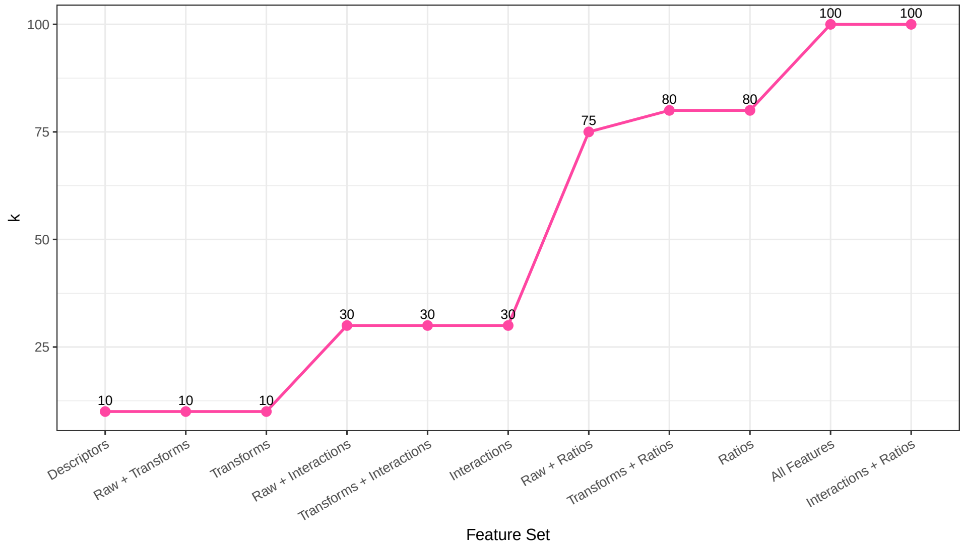
Optimal Feature Count across Feature Sets
