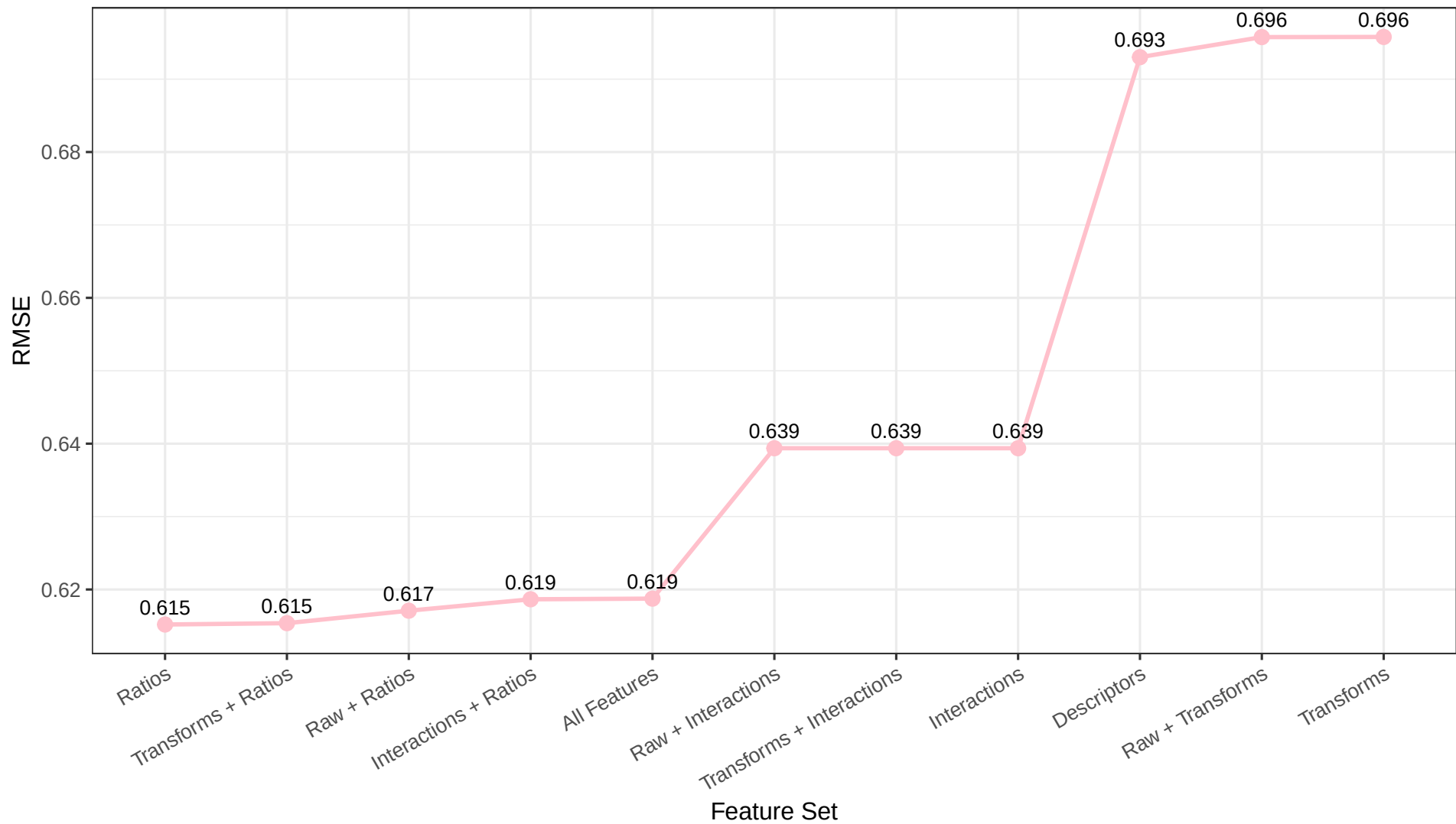
RMSE across Feature Sets
