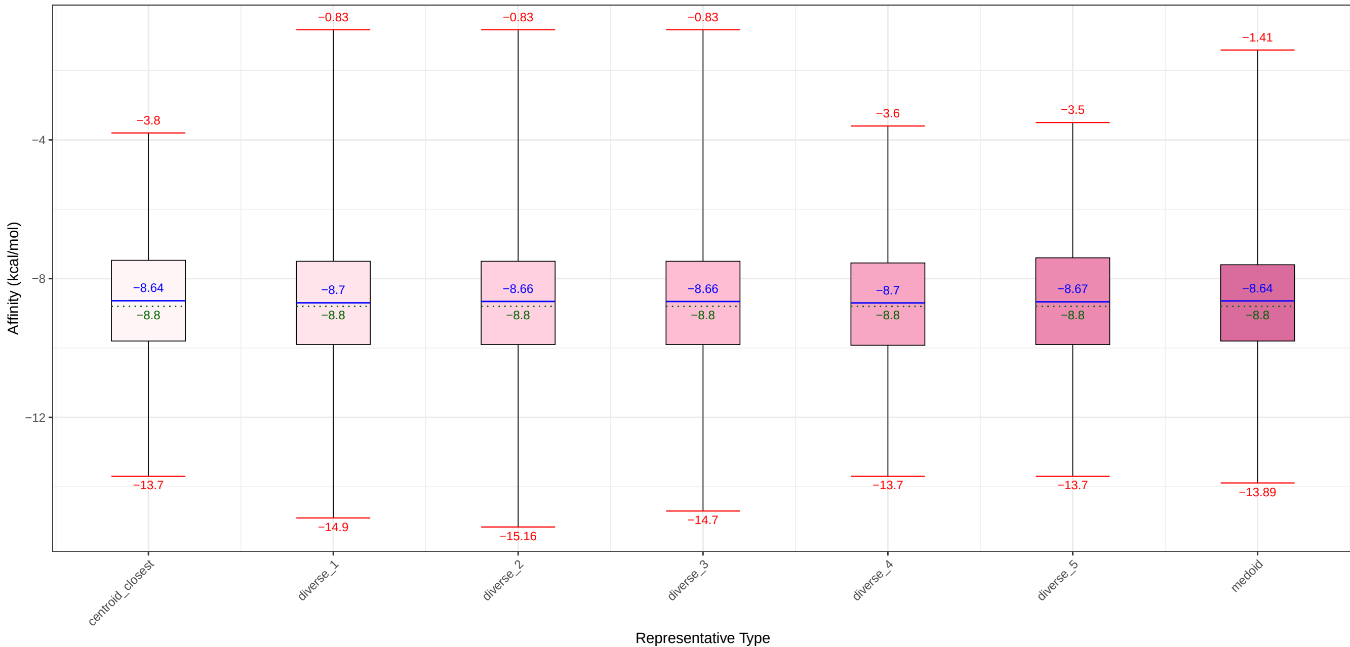
Docking Affinity Distribution of Representative Molecules against KEAP1
