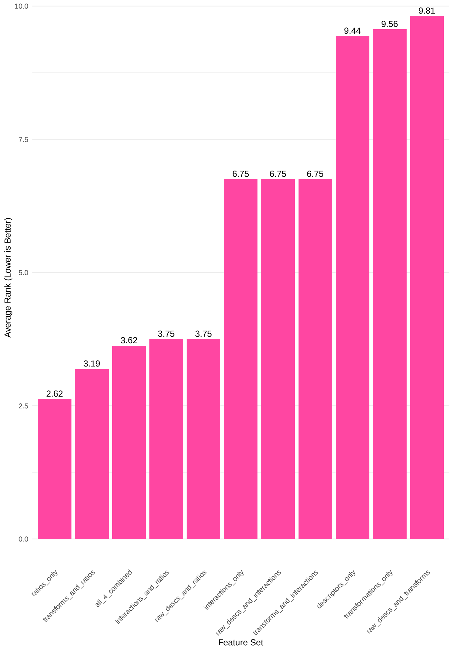
Feature Set Comparison (Average Rank)
