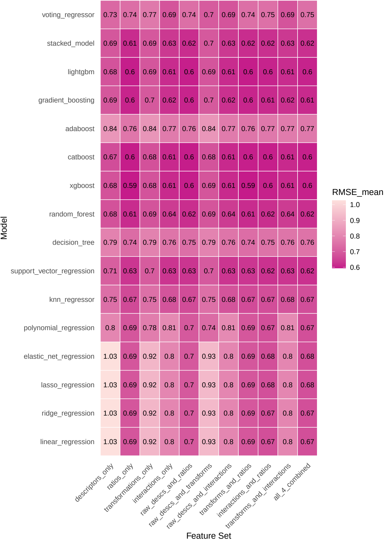
Mean RMSE across Models and Feature Sets
