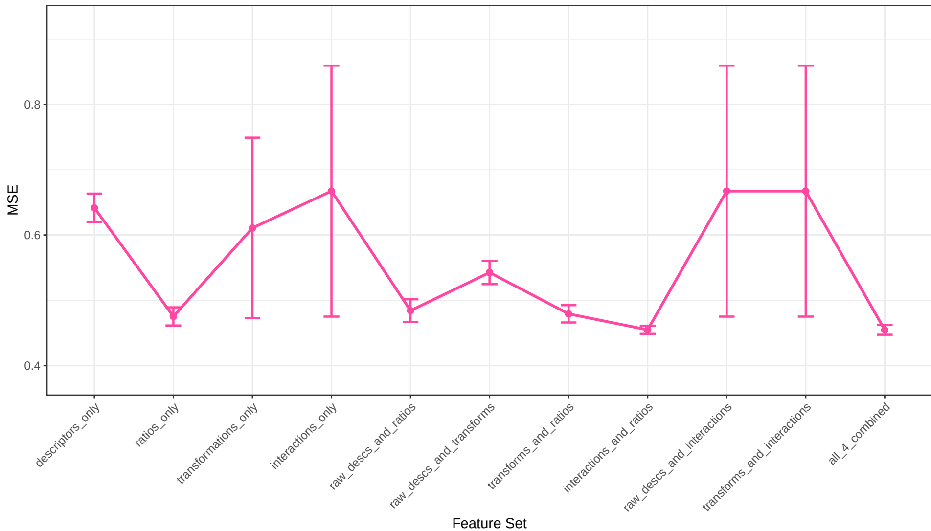
Polynomial Regression MSE Across Feature Sets
