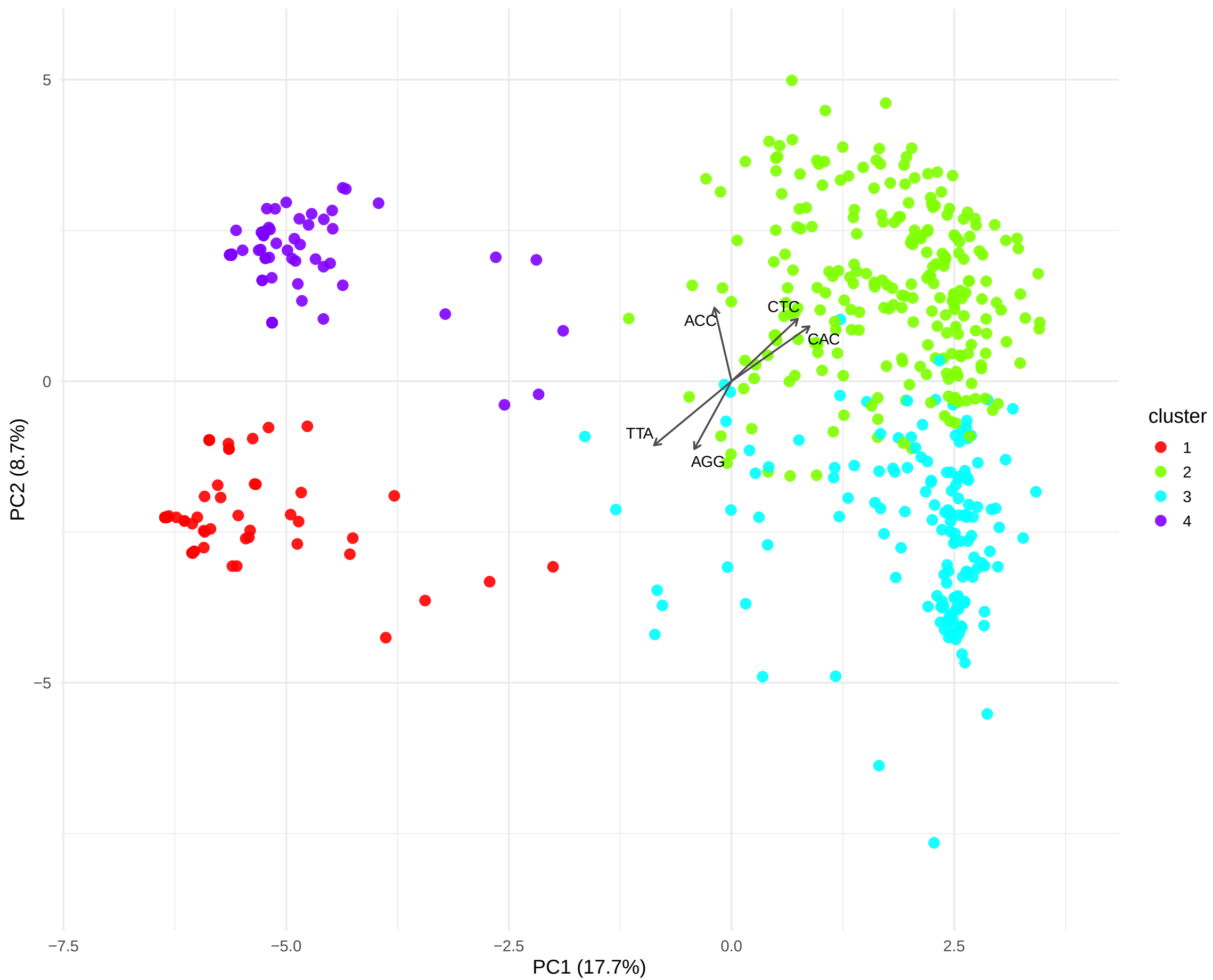
PC1 vs PC2 Colored by cluster
