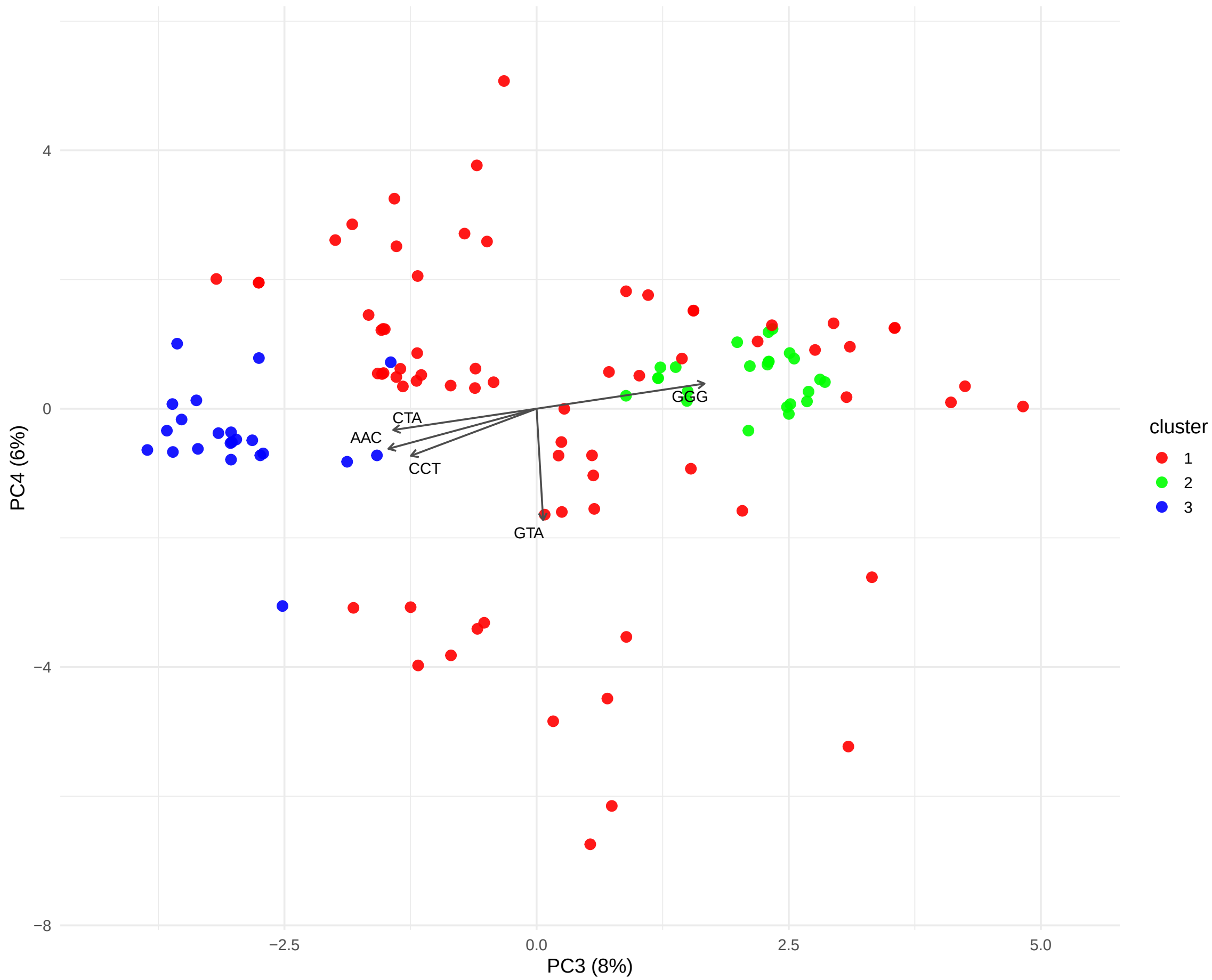
PC3 vs PC4 Colored by cluster
