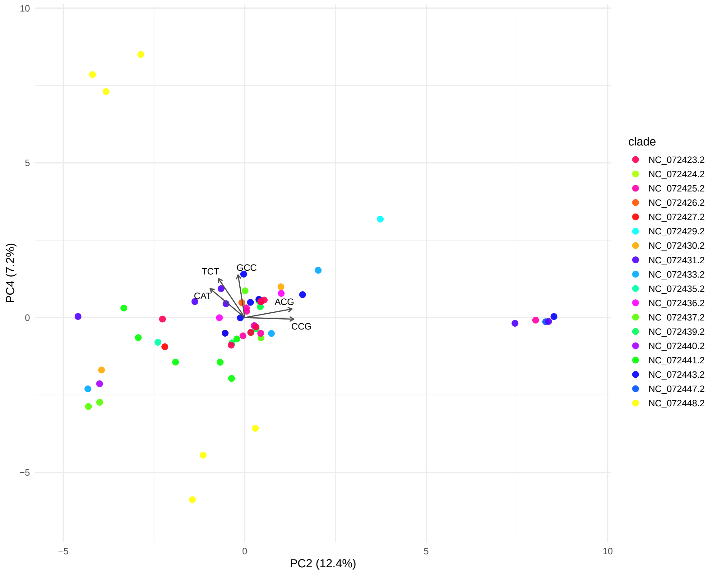
PC2 vs PC4 Colored by clade
