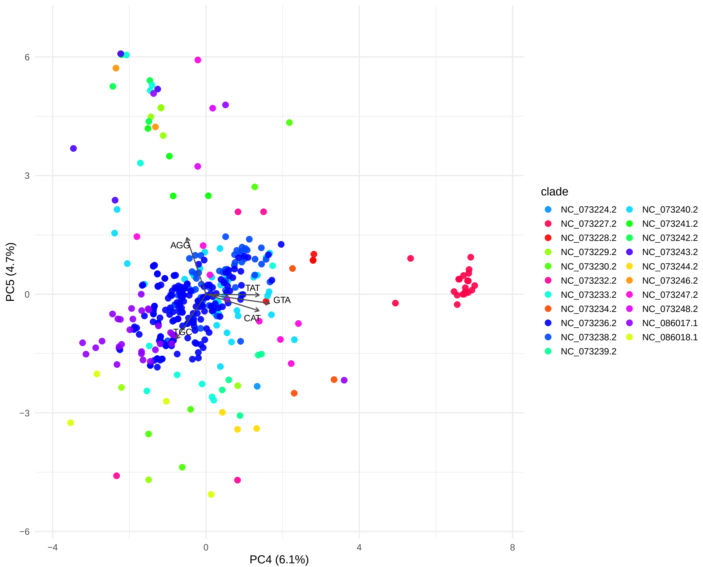
PC4 vs PC5 Colored by clade
