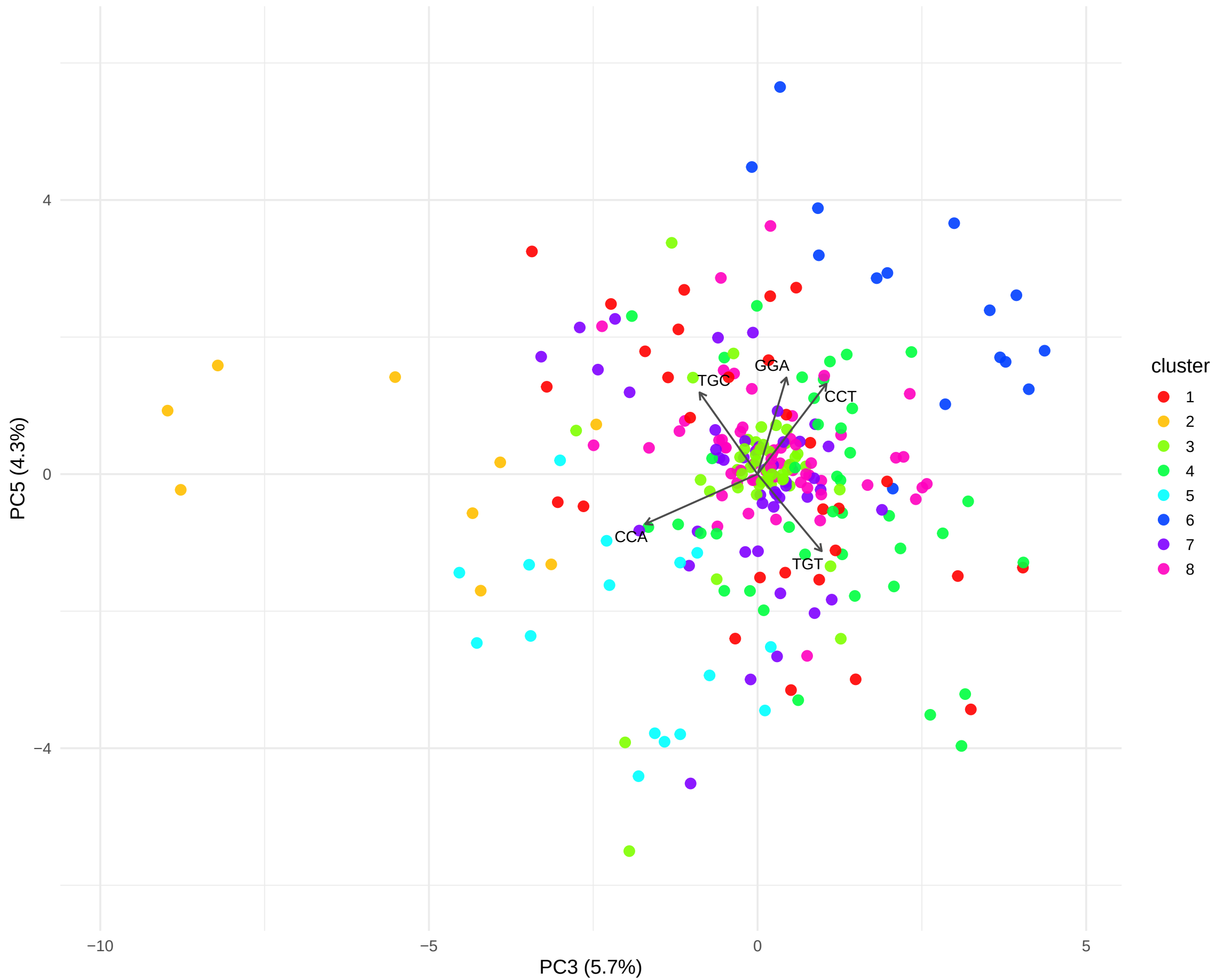
PC3 vs PC5 Colored by cluster
