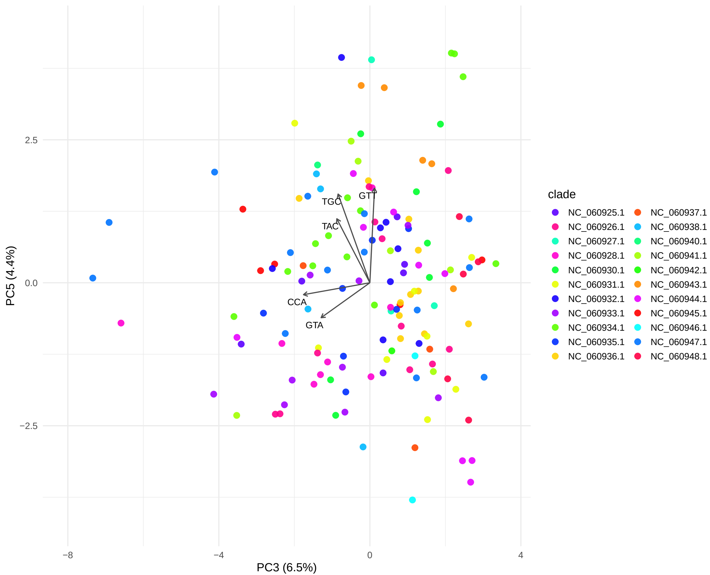
PC3 vs PC5 Colored by clade
