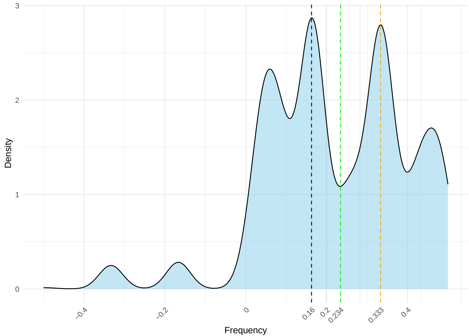
bonobo – SCFR Distribution
